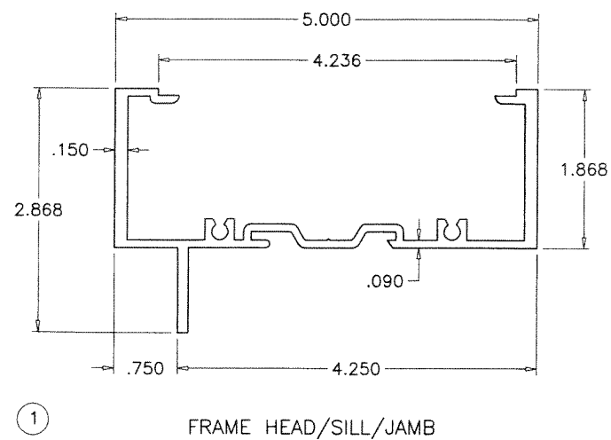
① FRAME HEAD/SILL/JAMB
