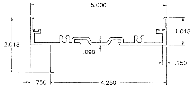
④ FEMALE FRAME
