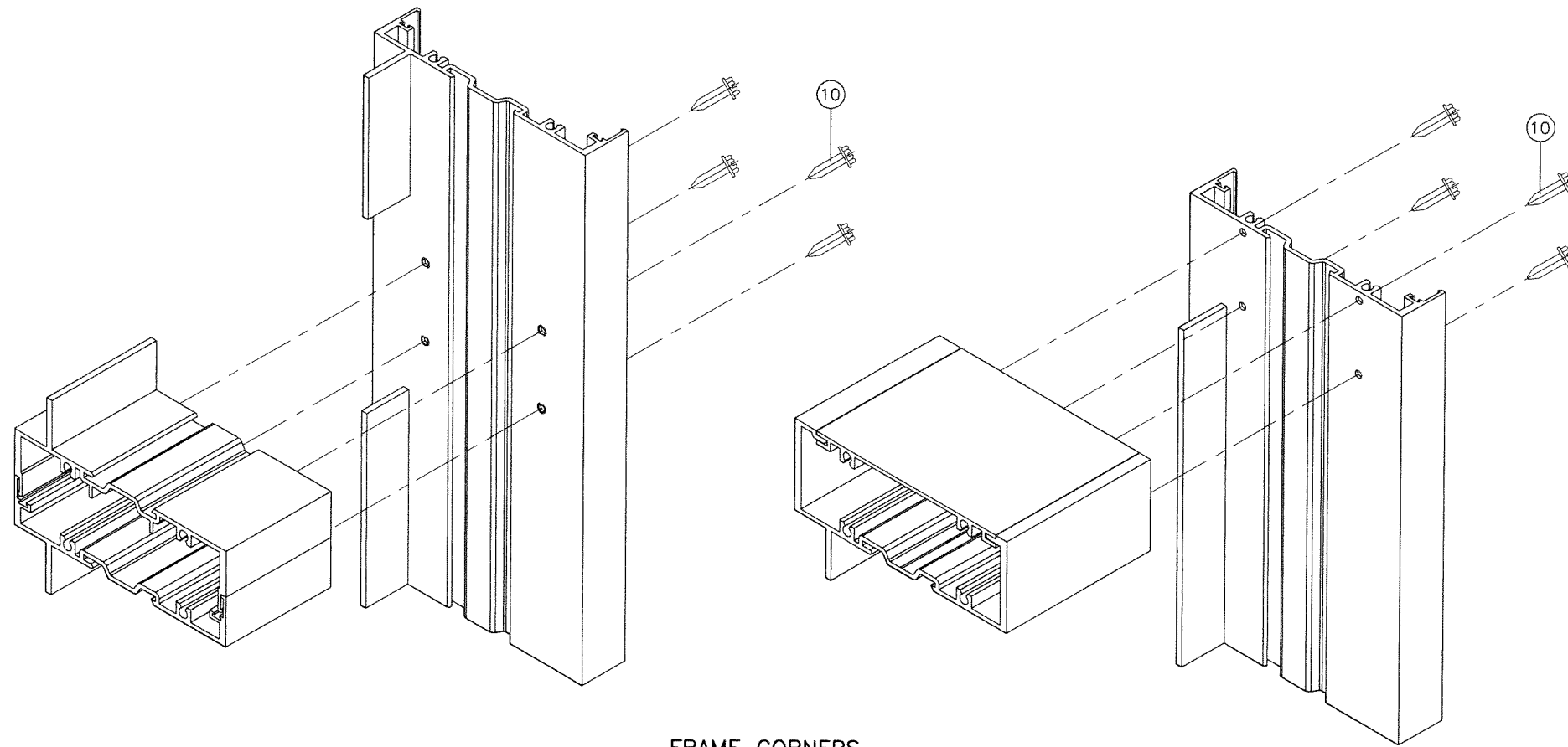
FRAME CORNERS
