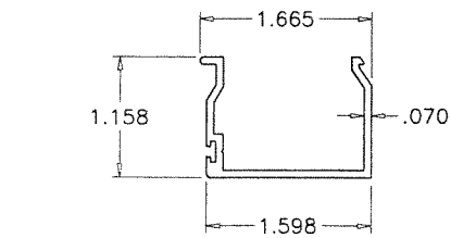
③ GLASS STOP (LAM. GLASS)
