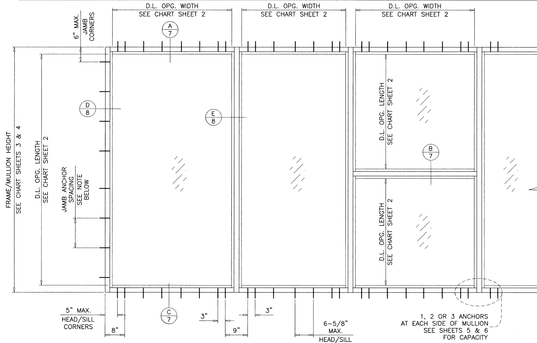
TYPICAL ELEVATIONS
