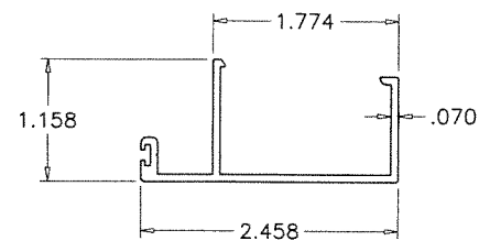
③A GLASS STOP (LAM. INSUL. GLASS)
